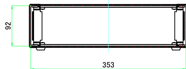
B-B (1:5)
