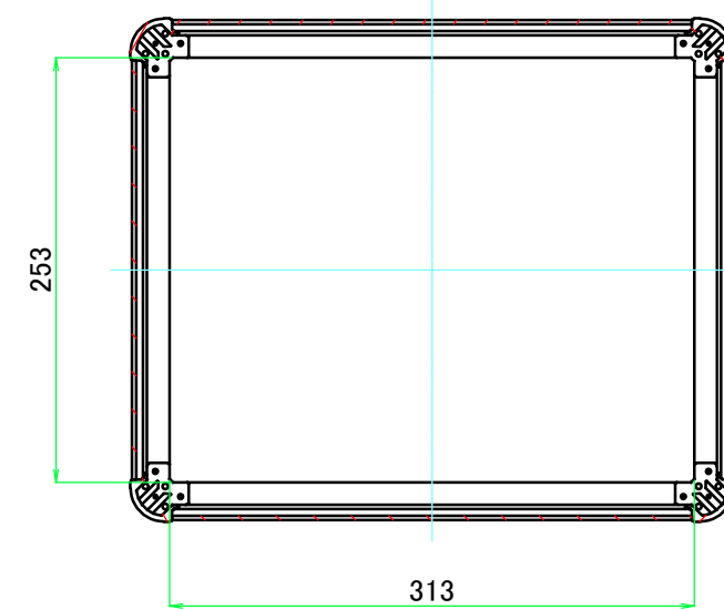
C-C (1:5)
